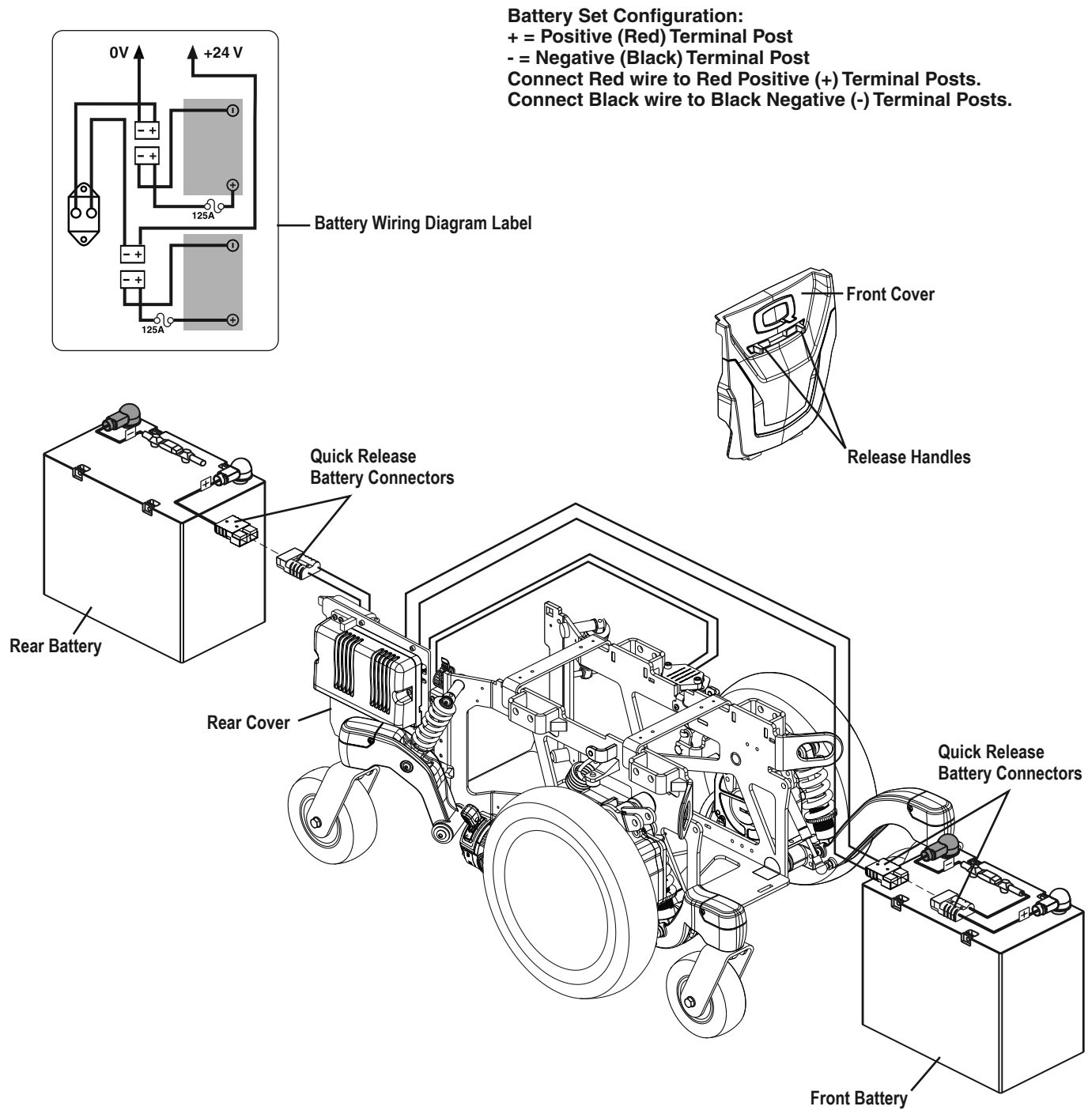
Figure 14. Battery Installation
